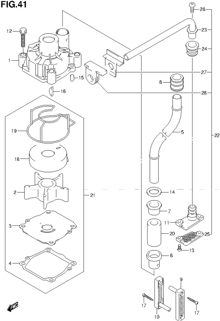
FIG.41 (1-E-6) WATER PUMP (DF115AZ E01)
