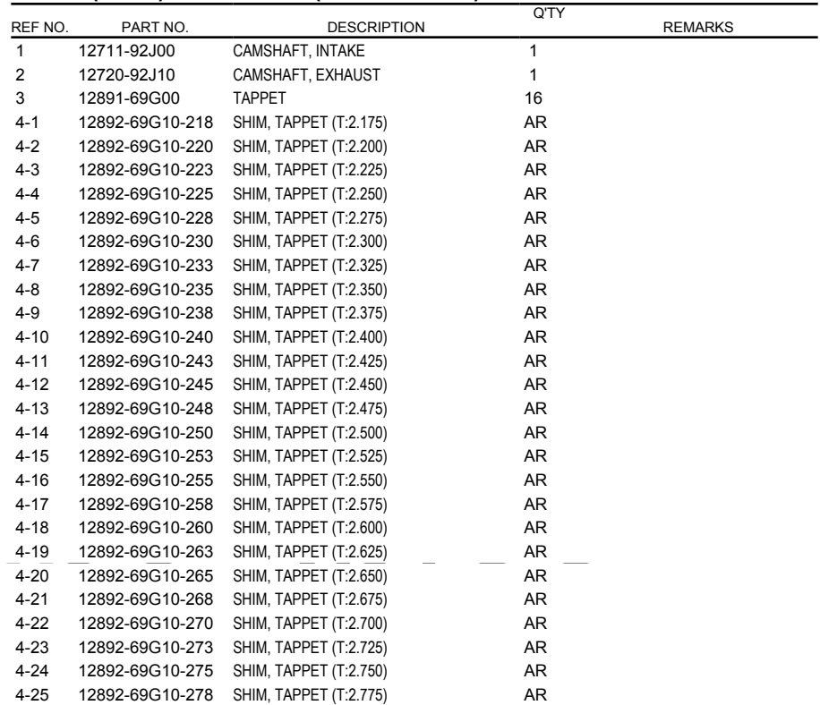
FIG.15 (1-C-6) CAMSHAFT (DF115AZ E01)
