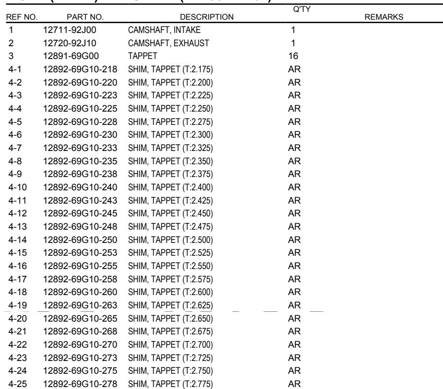
FIG.11 (1-B-12) CAMSHAFT (DF100AT E01)
