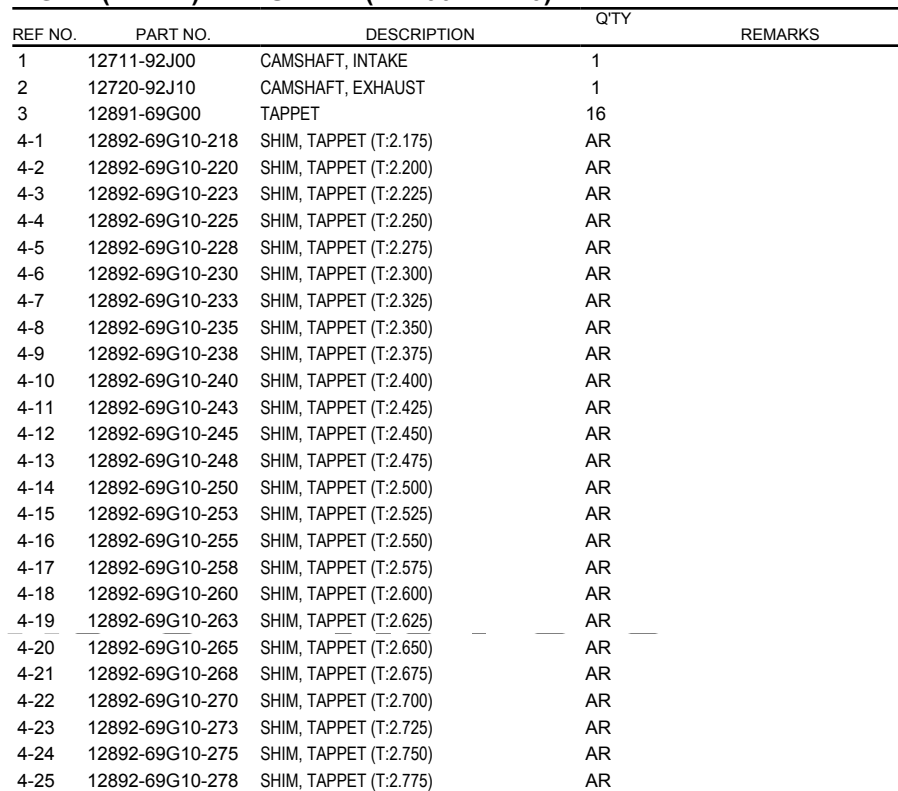
FIG.12 (1-B-14) CAMSHAFT (DF100AT E40)
