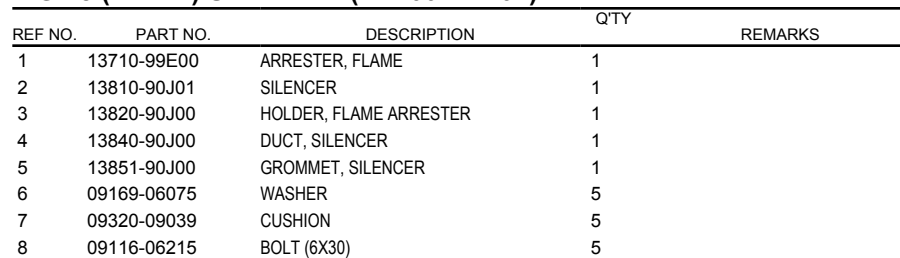
FIG.18 (1-C-11) SILENCER (DF100AT E01)
