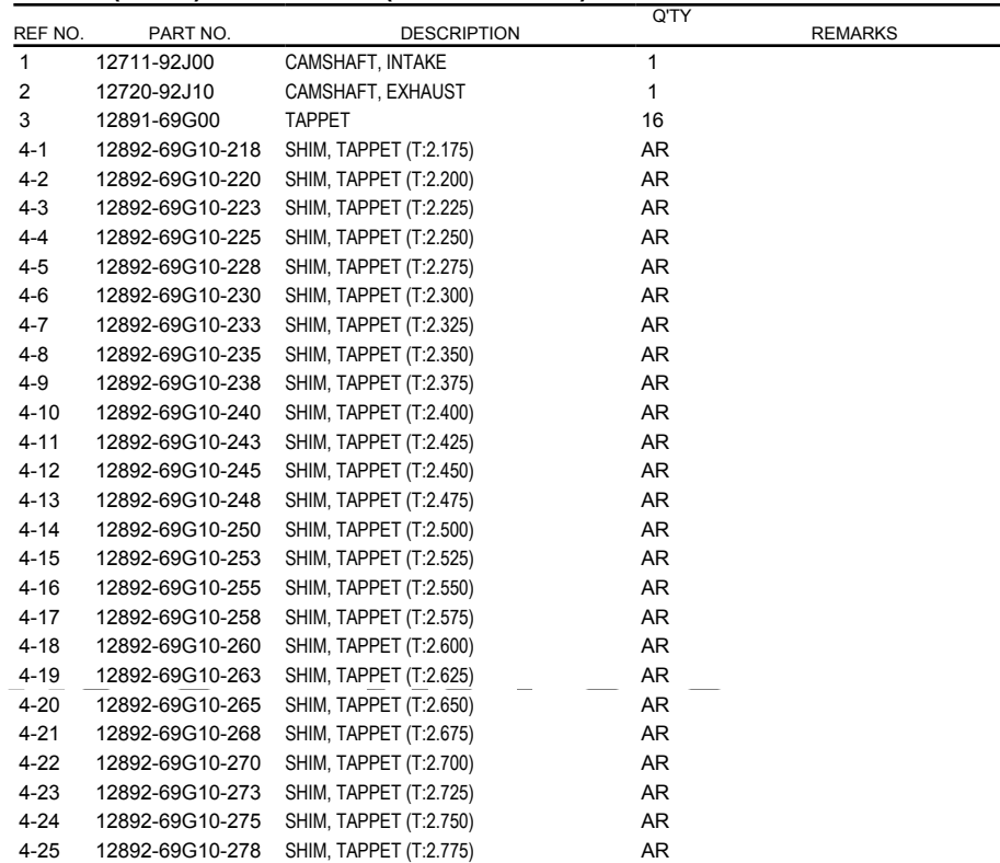
FIG.14 (1-C-4) CAMSHAFT (DF115AT E40)
