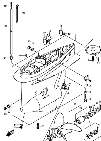
DF200AP_000_015_407A GEAR CASE
