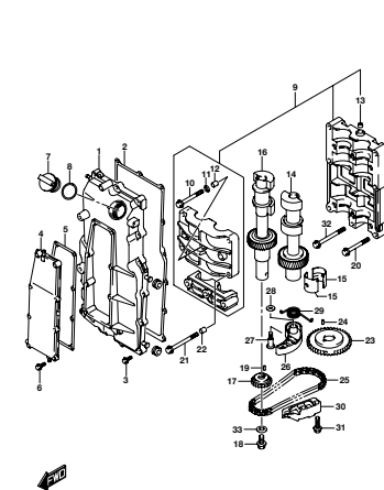
DF200AP_000_015_118A BALANCER
