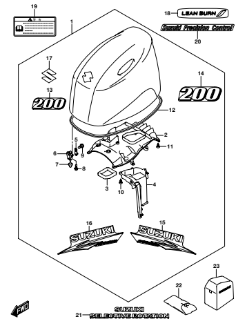
DF200AP_000_015_420A ENGINE COVER
