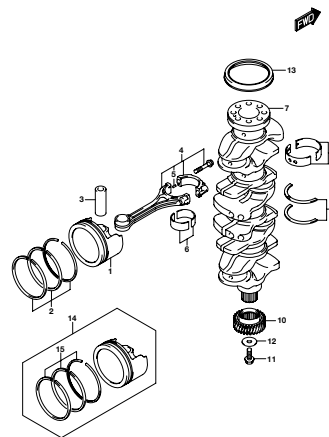
DF200AP_000_015_116A CRANKSHAFT
