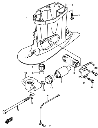
DF200AP_000_015_405A DRIVE SHAFT HOUSING
