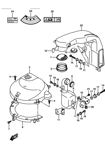
DF200AP_000_015_135A SILENCER/MUFFLER GEAR COVER
