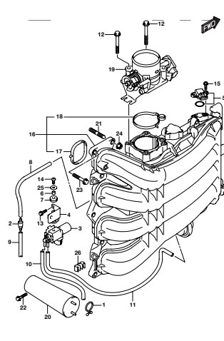
DF200AP_000_015_123A INTAKE MANIFOLD/THROTTLE BODY
