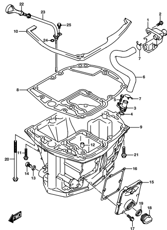
DF200AP_000_015_180A OIL PAN
