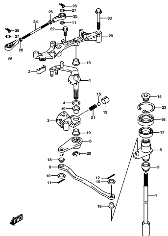
DF200AP_000_015_204A CLUTCH SHAFT
