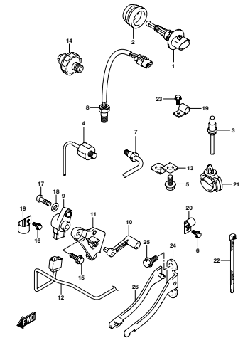
DF200AP_000_015_315A SENSOR
