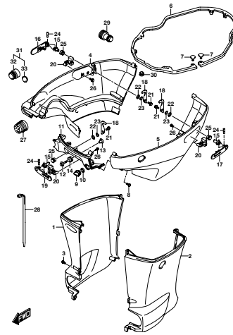
DF200AP_000_015_410A SIDE COVER
