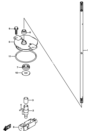
DF200AP_000_015_206A CLUTCH ROD
