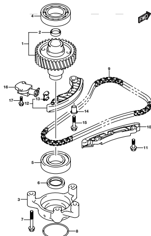
DF200AP_000_015_119A TIMING CHAIN
