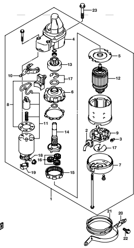
DF200AP_000_015_301A STARTING MOTOR
