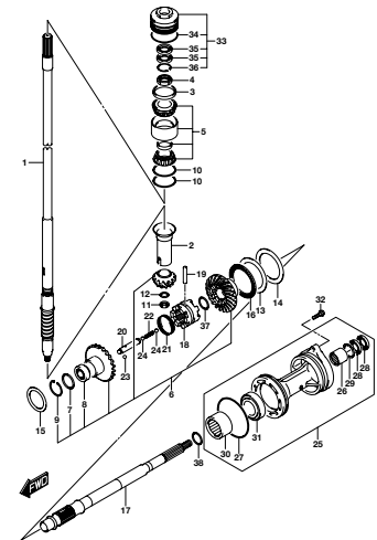
DF200AP_000_015_220A TRANSMISSION
