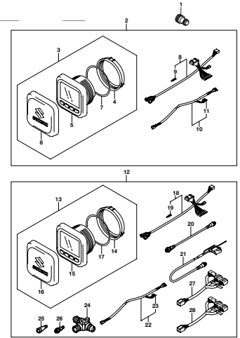
DF200AP_000_015_502A OPT-METER (1)
