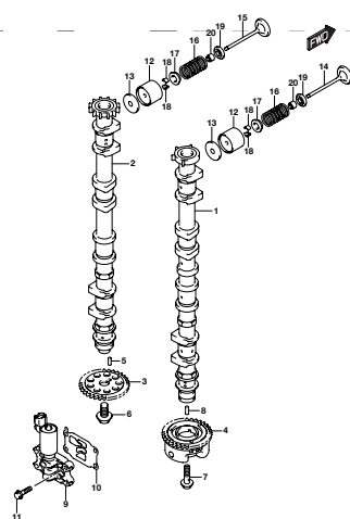
DF200AP_000_015_121A CAMSHAFT
