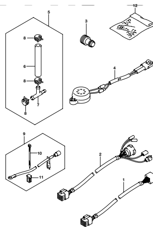
DF200A_000_016_522A OPT HARNESS (1)
