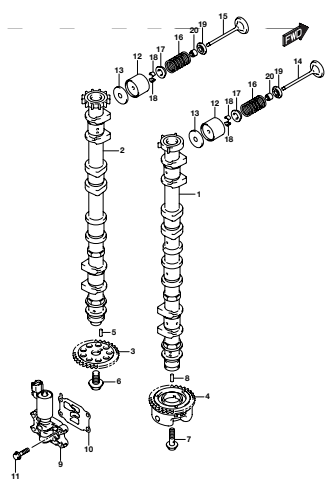
DF200A_000_016_121A CAMSHAFT
