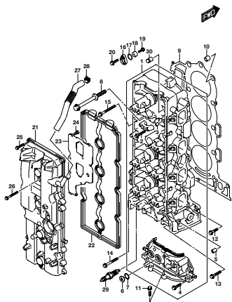
DF200A_000_016_111A CYLINDER HEAD
