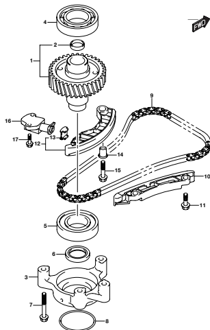
DF200A_000_016_119A TIMING CHAIN
