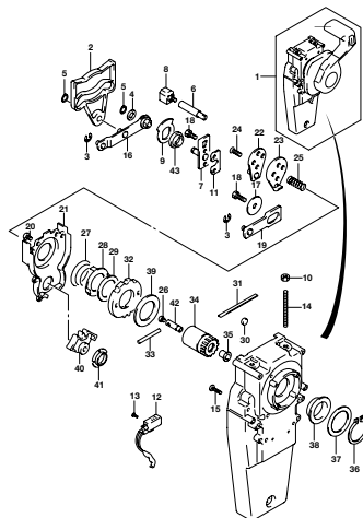
DF200A_000_016_518A OPT CONCEALED REMOCON (2)
