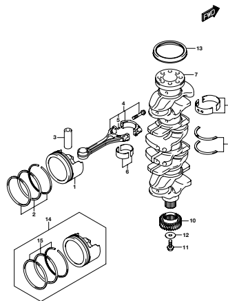
DF200A_000_016_116A CRANKSHAFT
