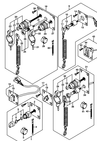
DF200A_000_016_530A OPT SWITCH
