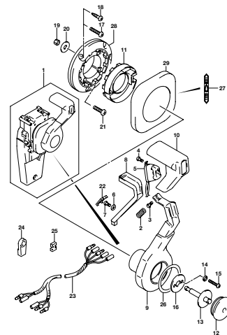
DF200A_000_016_517A OPT CONCEALED REMOCON (1)
