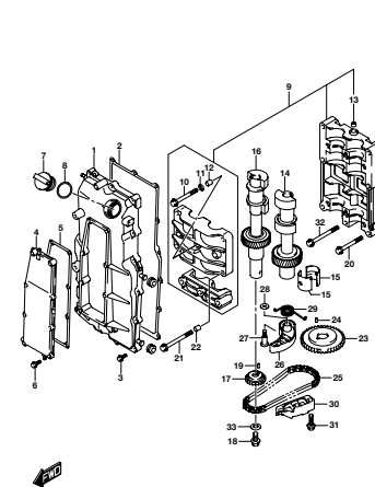
DF200A_000_016_118A BALANCER
