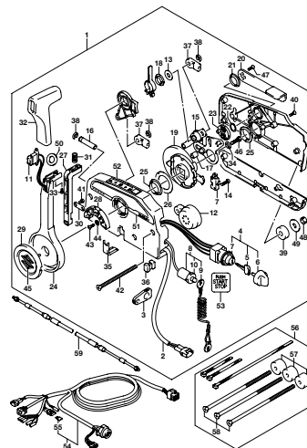
DF200A_000_016_508A OPT REMOTE CONTROL
