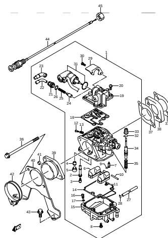
DF25 000_006 CARBURETOR-C
