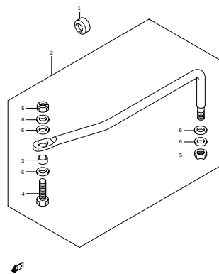
DF25 000_033 DRAG LINK (TYPE R)-C
