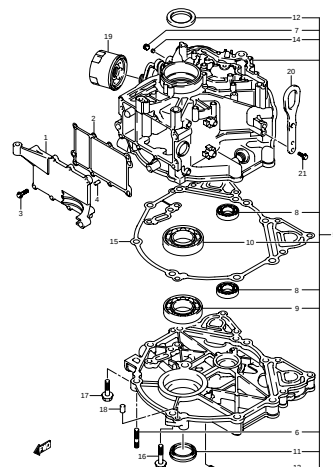
DF25 000_002 CYLINDER BLOCK-C
