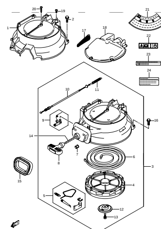
DF25 000_007 MAGNETO COVER/RECOIL/SILENCER
