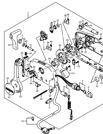
DF25 000_034 REMOTE CONTROL BOX-C
