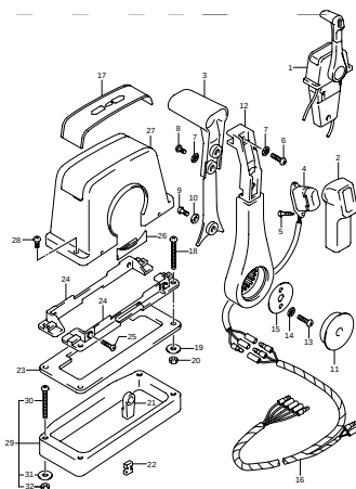
DF25 000_037 OPT-TOP MOUNT SINGLE (1)-C
