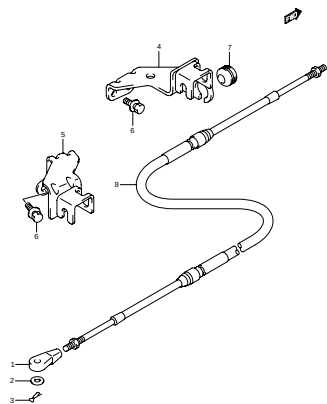
DF25 000_032 REMOCON CABLE (TYPE R)-C
