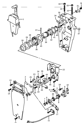
DF25 000_038 OPT-TOP MOUNT SINGLE (2)-C
