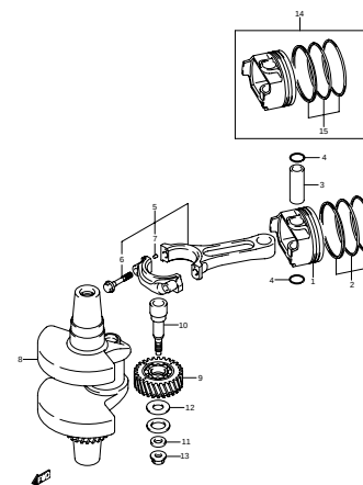
DF25 000_003 CRANKSHAFT-C
