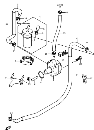
DF25 000_008 FUEL PUMP-C
