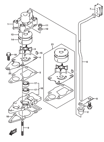
DFSA_GA_NOD_019_160A WATER PUMP
