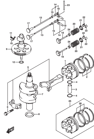
DFSA_GA_NOD_019_116A CRANKSHAFT
