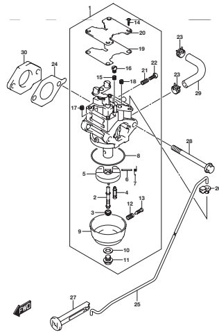
DFSA_GA_NOD_019_128B CARBURETOR
