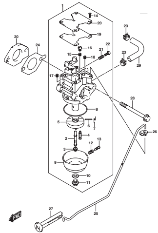
DFSA_GA_NOD_019_128A CARBURETOR
