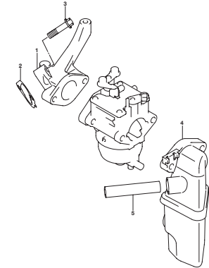
DFSA_GA_NOD_019_122A INTAKE MANIFOLD
