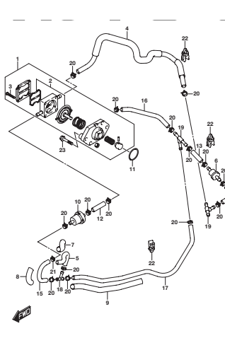
DFSA_GA_NOD_019_146A FUEL PUMP
