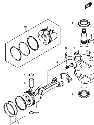
DFSA_S/SA_NKD_015_116A CRANKSHAFT
