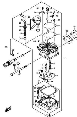
DFSA_S/SA_NKD_015_128B CARBURETOR
