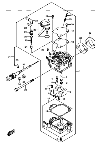
DFSA_S/SA_NKD_015_128A CARBURETOR
