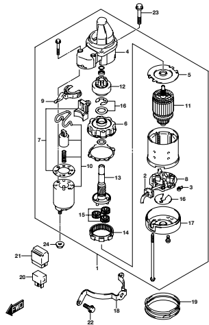
DPF SA_NKD_017_301A STARTING MOTOR
