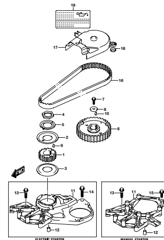
DF9 SA_MNO_017_120A TIMING BELT
