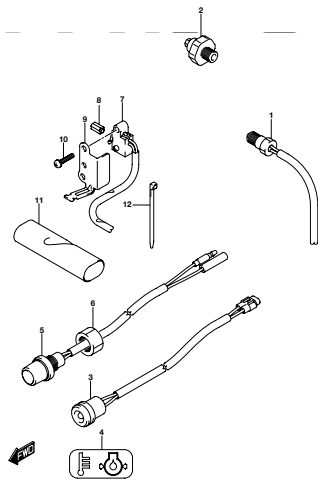
DPF SA_NKD_017_334A SENSOR/SWITCH
