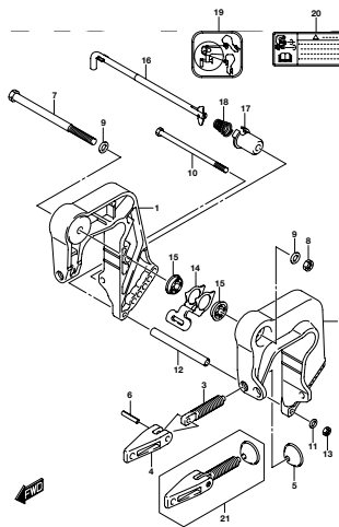
DPF SA_NKD_017_335A CLAMP BRACKET
