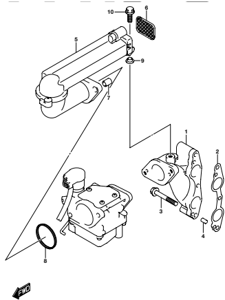
DF9 SA_MNO_017_126A INLET MANIFOLD
