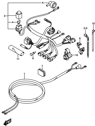
DPF SA_NKD_017_322A HARNESS
