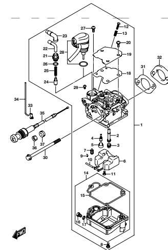
DF9 SA_MNO_017_128A CARBURETOR
