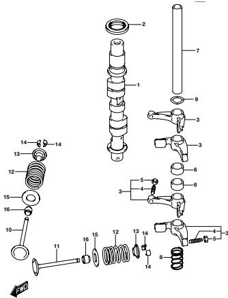
DF9 SA_MNO_017_121A CAMSHAFT
