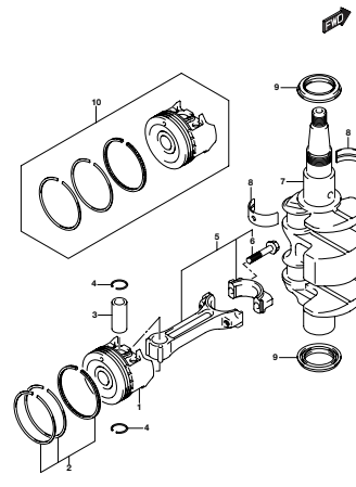
DF9 SA_MNO_017_116A CRANKSHAFT
