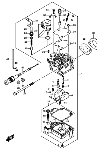
DF9 SA_MNO_017_128B CARBURETOR
