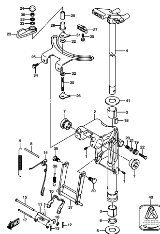
DPF SA_NKD_017_336A SWIVEL BRACKET
