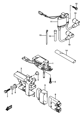
DPF SA_NKD_017_310A RECTIFIER/IGNITION COIL
