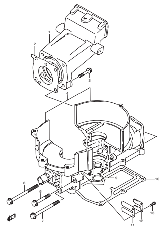
DT2.2 000_001 CYLINDER
