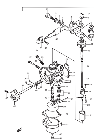
DT2.2 000_003 CARBURETOR
