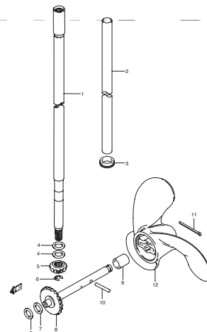
DT2.2 000_006 TRANSMISSION
