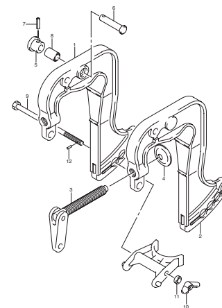
DT2.2 000_008 CLAMP BRACKET
