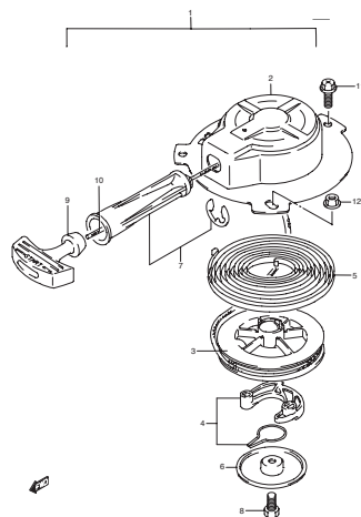
DT2.2 000_005 RECOIL STARTER
