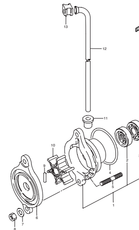
DT2.2 000_004 WATER PUMP
