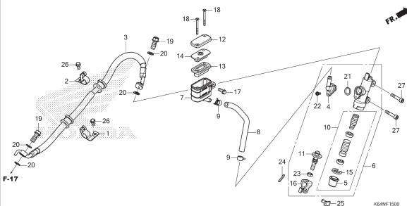
F-15 REAR BRAKE MASTER CYLINDER (CBR250S3)
