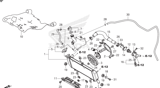
F-41 RADIATOR
