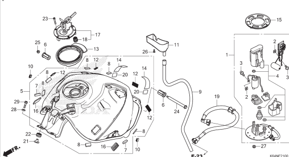
F-21 FUEL TANK/FUEL PUMP
