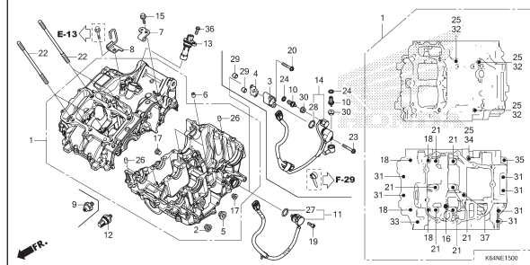
E-15 CRANKCASE
