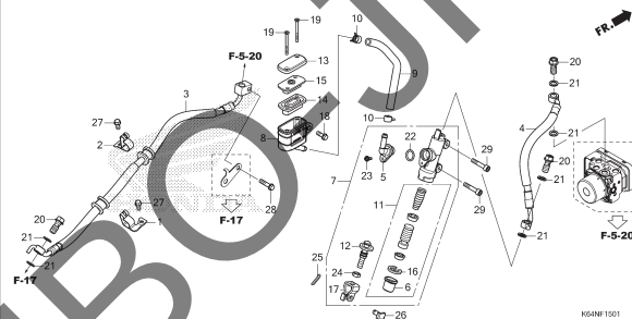
F-15-1 REAR BRAKE MASTER CYLINDER (CBR250S3A)
