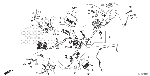
F-38 WIRE HARNESS
