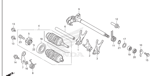
E-19 GEARSHIFT DRUM
