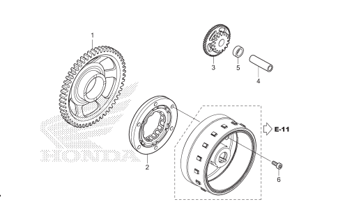
E-9 STARTING CLUTCH
