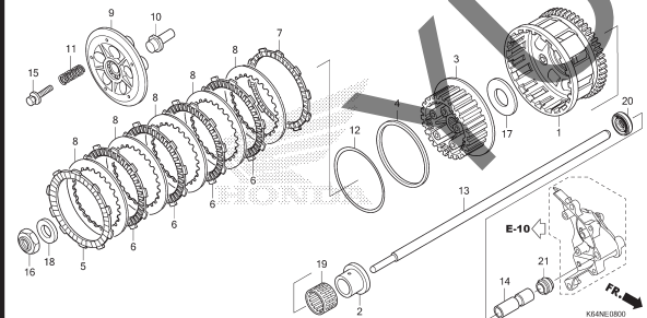
E-8 CLUTCH(CBR250S3)
