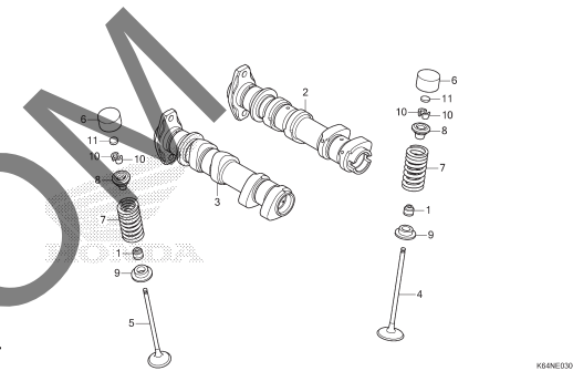
E-3 CAMSHAFT/VALVE
