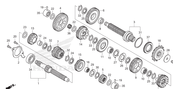
E-17 TRANSMISSION
