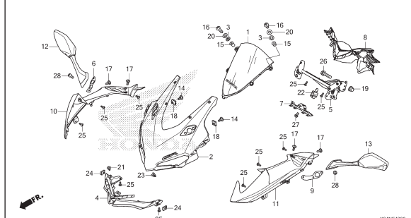
F-43 UPPER COWL
