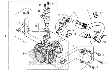
THROTTLE BODY
