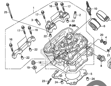
CYLINDER
