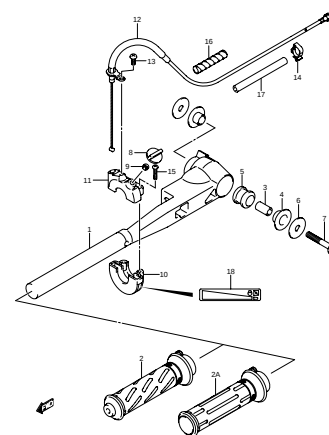
DF2 N00_020 TILLER HANDLE
