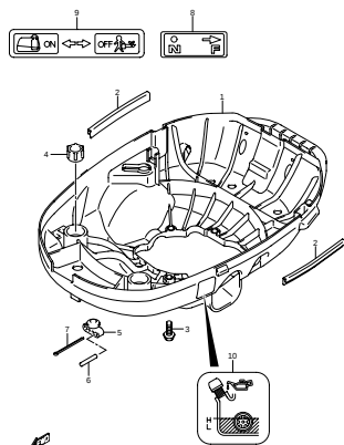
DF2 N00_017 LOWER COVER-C
