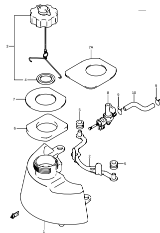
DF2 N00_021 FUEL TANK
