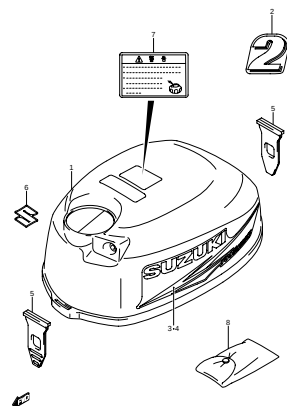
DF2 N00_019 ENGINE COVER (MODEL:10)
