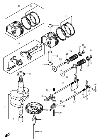
DF2 N00 013_003 CRANKSHAFT
