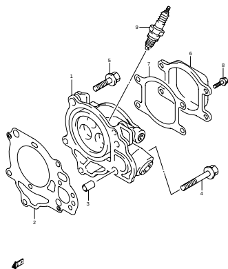
DF2 N00 013_001 CYLINDER HEAD
