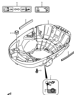
DF2 N00 013_017 LOWER COVER
