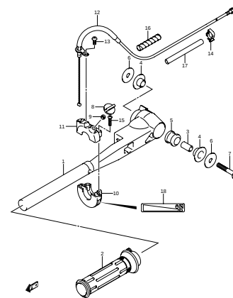
DF2 N00 013_019 TILLER HANDLE
