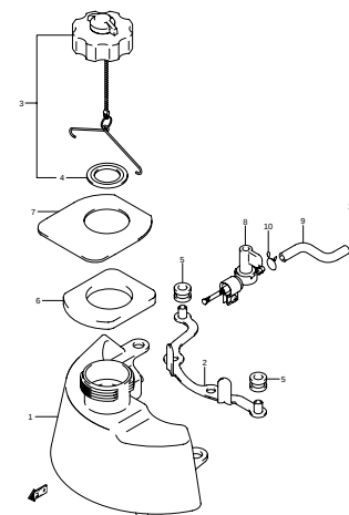
DF2 N00 013_020 FUEL TANK
