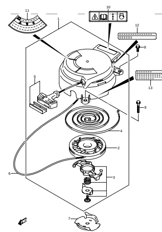
DF2 N00 013_007 RECOIL STARTER
