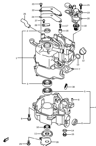
DF2 N00 013_002 CYLINDER BLOCK
