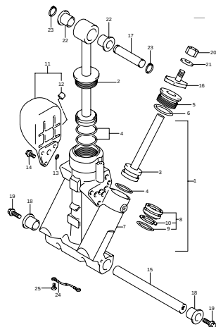
DF200 225 250 000_036 TRIM CYLINDER (DF200TL)-C
