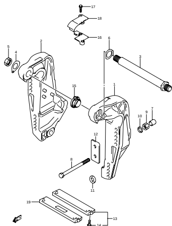
DF200 225 250 000_032 CLAMP BRACKET (DF200TL)-C
