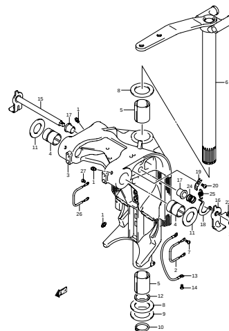
DF200 225 250 000_034 SWIVEL BRACKET (DF200TL)-C
