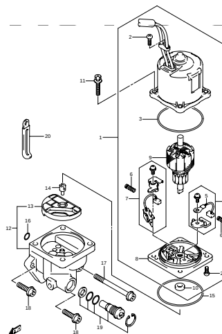
DF200 225 250 000_038 PTT MOTOR (DF200TL)-C
