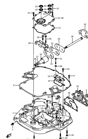
DF200 225 250 000_039 ENGINE HOLDER
