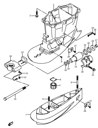
DF300A_000_014_031 DRIVE SHAFT HOUSING
