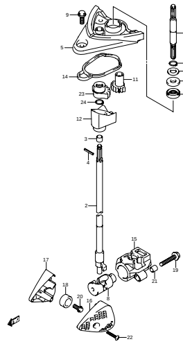
DF300A_000_014_017 CLUTCH ROD
