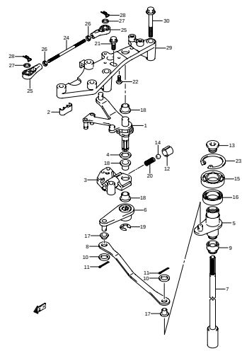
DF300A_000_014_016A CLUTCH SHAFT
