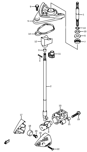
DF300A_000_014_017A CLUTCH ROD
