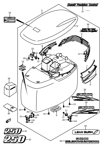
DF300A_000_014_035 ENGINE COVER
