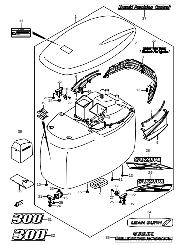
DF300A_000_014_034 ENGINE COVER
