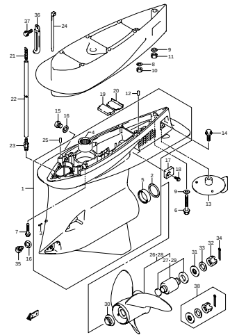
DF300A_000_014_032 GEAR CASE
