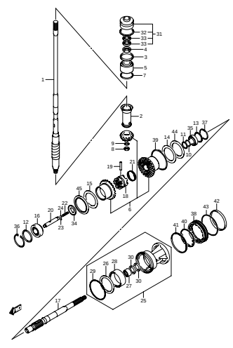
DF300A_000_014_018 TRANSMISSION
