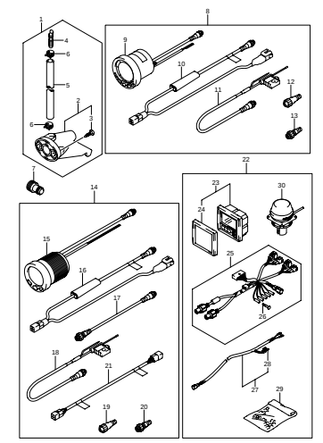
DF300A_000_014_038 OPTOMETER (1)
