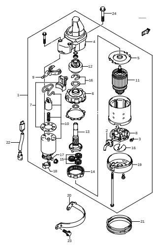
DF300A_000_014_019 STARTING MOTOR
