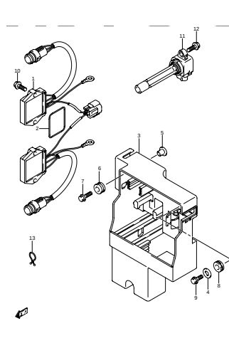
DF300A_000_014_021 RECTIFIER/IGNITION COIL
