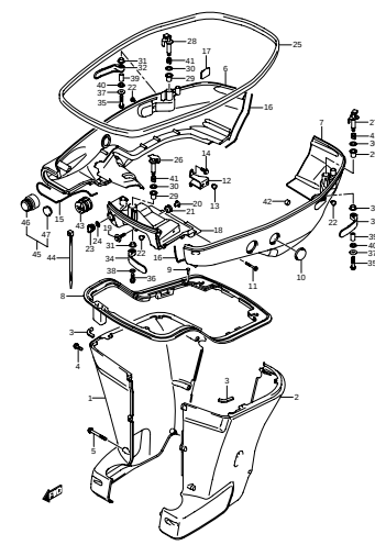
DF300A_000_014_033 SIDE COVER
