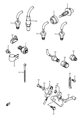
DF300A_000_014_022 SENSOR
