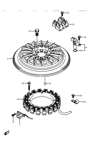
DF300A_000_014_020 MAGNETO
