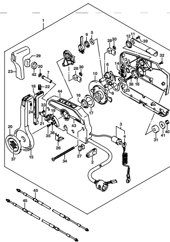
DFI, NO. 015_508A OPT REMOTE CONTROL
