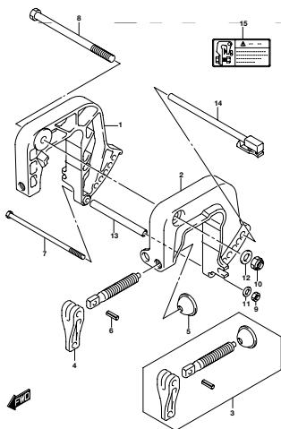
DFI, MOD. 015_335A CLAMP BRACKET
