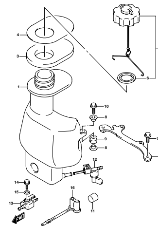
DFI, NO. 015_432A FUEL TANK
