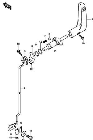
DFI, MOD. 015_208A CLUTCH LEVER
