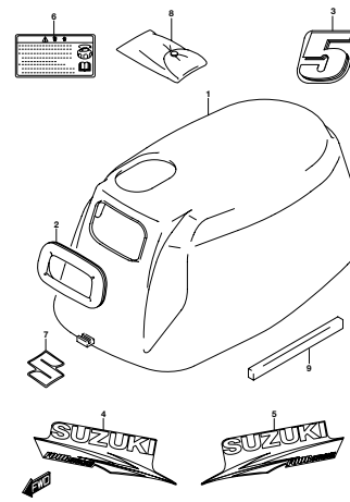
DFI, NO. 015_420A ENGINE COVER
