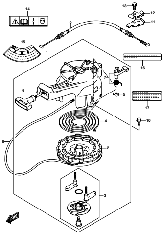
DFI, MOD. 015_167A RECOIL STARTER
