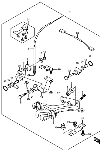
DFI, NO. 015_514A OPT REMOCON PARTS SET
