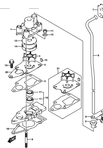
DFL_MOD_016_160A WATER PUMP
