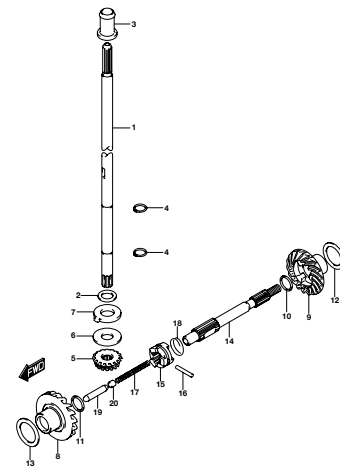
DFI, MOD. 015_230A DRIVE SHAFT
