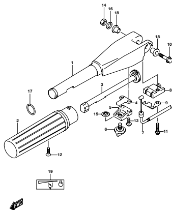
DFI, NO. 015_444A TILLER HANDLE
