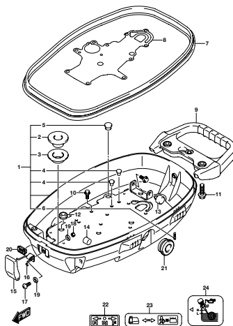
DFI, NO. 015_412A LOWER COVER
