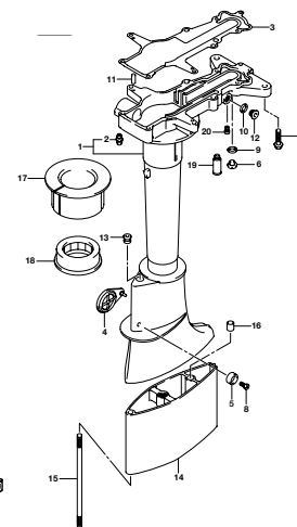
DFI, MOD. 015_405A DRIVE SHAFT HOUSING
