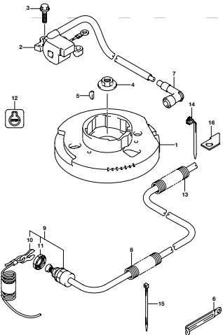
DFI, MOD. 015_303A MAGNETO
