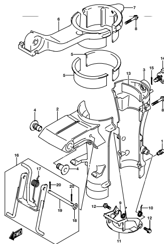
DFI, MOD. 015_336A SHIMEL BRACKET
