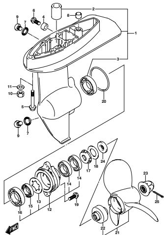
DFI, NO. 015_407A GEAR CASE
