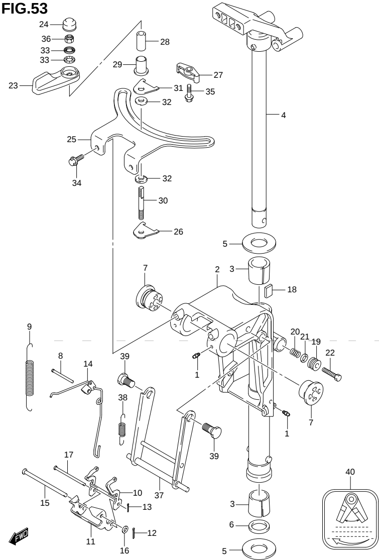
DF8A 9.9A P03 012_053 SWIVEL BRACKET
