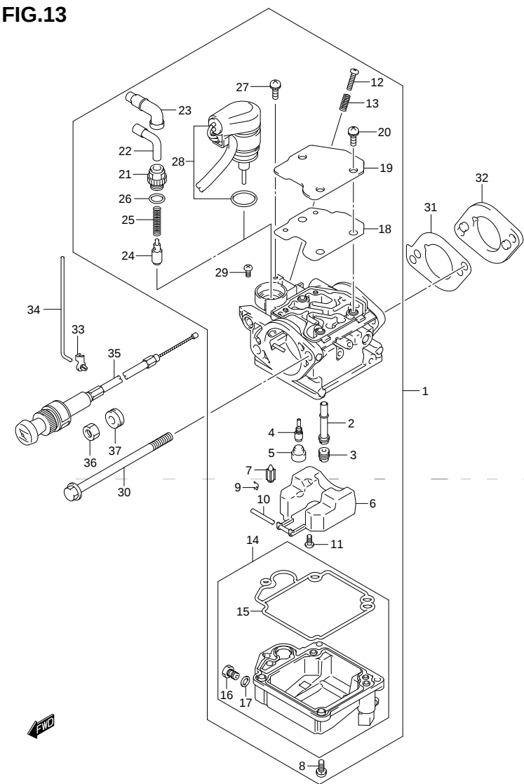
FIG.13 (1-B-15) CARBURETOR (DF8A P03)
