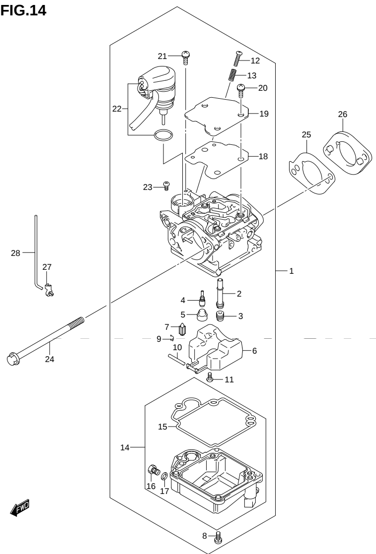
FIG.14 (1-C-2) CARBURETOR (DF8AR P03)
