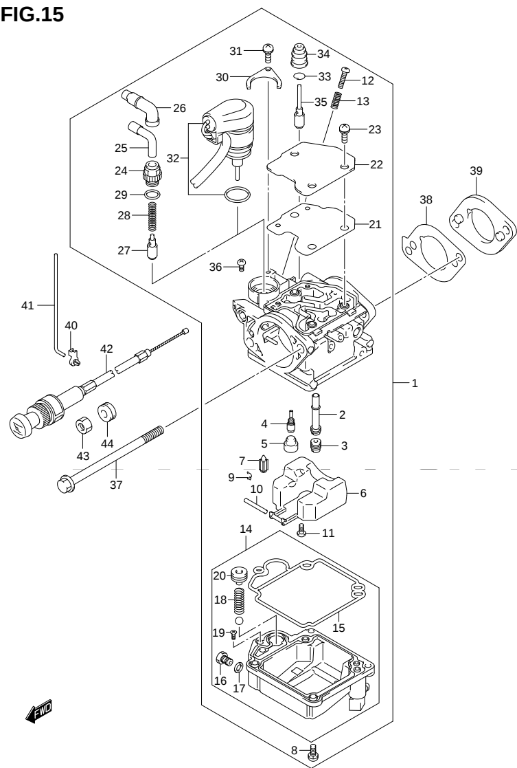
DF8A 9.9A P03 012_015 CARBURETOR
