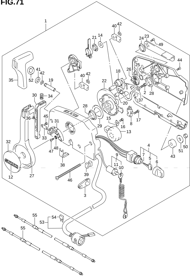
DF8A 9.9A P03 012_071 REMOTE CONTROL
