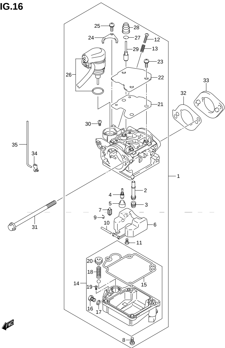
FIG.16 (1-C-5) CARBURETOR (DF15AR P03)
