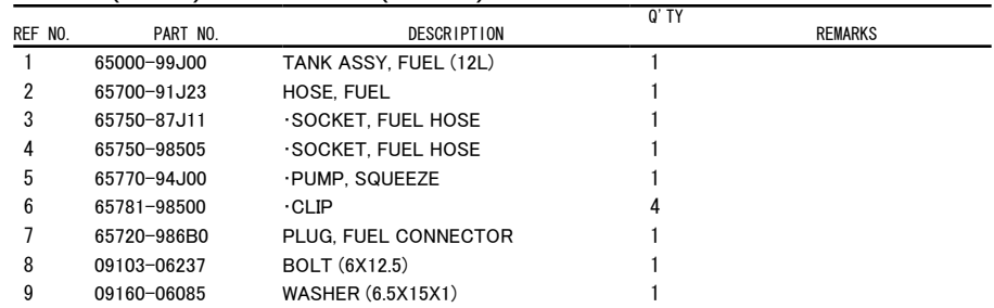
FIG.68 (1-G-6) FUEL TANK (RESIN)
